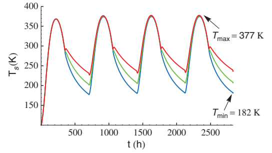
Fig. 7 Influence of nighttime heat-loss-limiting radiation shield on the thermal wadi-surface temperature vs time for a 50-cm-deep wadi with the thermal properties of basalt rock. \epsilon_0 = 0.9 during daytime for all curves (blue curve: \epsilon_1 = 0.9 ; green curve: \epsilon_1 = 0.5 ; red curve: \epsilon_1 = 0.25 ).
