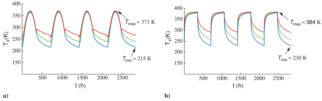
Fig. A1 Periodic steady-state surface temperature calculated employing Jaeger's method [8] for an infinitely deep basalt layer for a) sinusoidal heat flux and b) a square wave heat flux. Peak flux = 1300 \text{ W/m}^2 . \epsilon_0 = 0.9 during daytime for all curves (blue curve: \epsilon_1 = 0.9 ; green curve: \epsilon_1 = 0.5 ; red curve: \epsilon_1 = 0.25 ).
