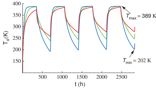
Fig. 9 The effect of wadi depth on the surface temperature of an equatorial thermal wadi with a solar reflector, a heat-loss-limiting radiation shield, and rover heating [25 cm (blue), 50 cm (green), and 100 cm (red), each with the thermal properties of basalt].
