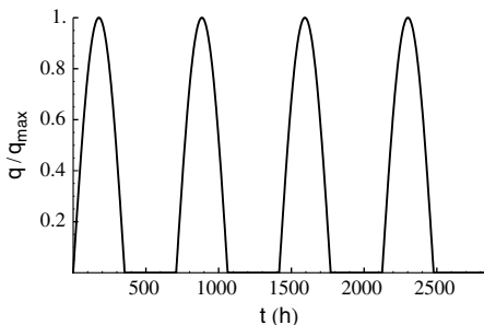
Fig. 2 Equatorial solar flux. The solar flux profile is a semisinusoid.
