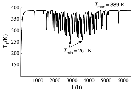
Fig. 13 Same as Fig. 12 but without the heat-loss-limiting shield.
