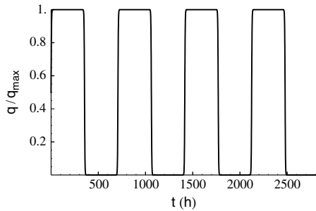
Fig. 3 Equatorial solar flux obtained with the use of a sun-tracking reflector. The solar flux profile is a square wave.
