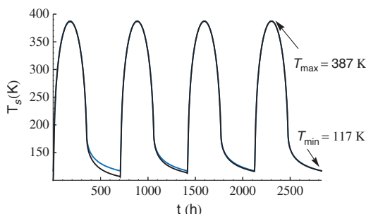
Fig. 6 Surface temperature vs time for native regolith. The equatorial solar flux is as shown in Fig. 2 (black curve: present calculations for a 20-cm-deep layer; blue curve: periodic steady-state result calculated using Jaeger's method [8] for an infinitely deep layer).
