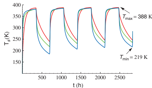
Fig. 10 The effect of thermal diffusivity on the surface temperature of an equatorial thermal wadi with a solar reflector, a heat-loss-limiting radiation shield, and rover heating for a 50-cm-deep wadi [basalt value (red), one-fifth of basalt value (green), and one-tenth of basalt value (blue)].
