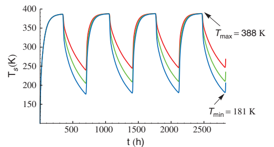
Fig. 8 Surface temperature of an equatorial thermal wadi with a solar reflector, a heat-loss-limiting radiation shield, and rover heating for a 50-cm-deep wadi [ \epsilon_1 = 0.9 (blue), \epsilon_1 = 0.5 (green), and \epsilon_1 = 0.25 (red)].
