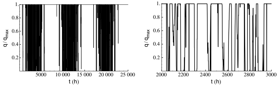
Fig. 5 Solar flux at the polar site with the use of a reflector.
