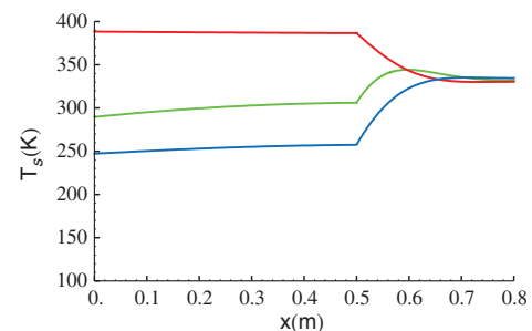
Fig. 11 Temperature distribution vs distance below the surface for a 50-cm-deep wadi and a 30-cm-deep underlying regolith layer. The solar flux is as shown in Fig. 3, with 12 diurnal cycles, q_{\text{rov}} = 25 \text{ W/m}^2 [ t = 8127 \text{ h} (red), t = 8307 \text{ h} (green), and t = 8486 \text{ h} (blue)].
