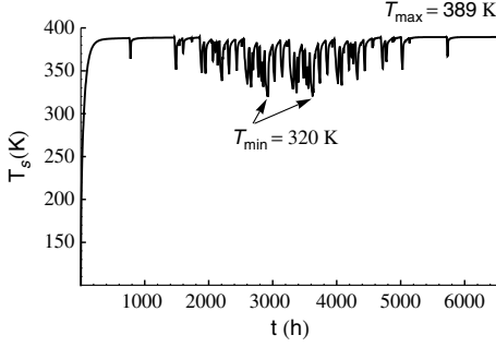
Fig. 12 Surface temperature of the thermal wadi of depth 50 cm, with thermal properties of basalt rock at the lunar polar site using the sun-tracking reflector and the heat-loss-limiting shield. Heat is supplied to a rover during the periods of darkness.
